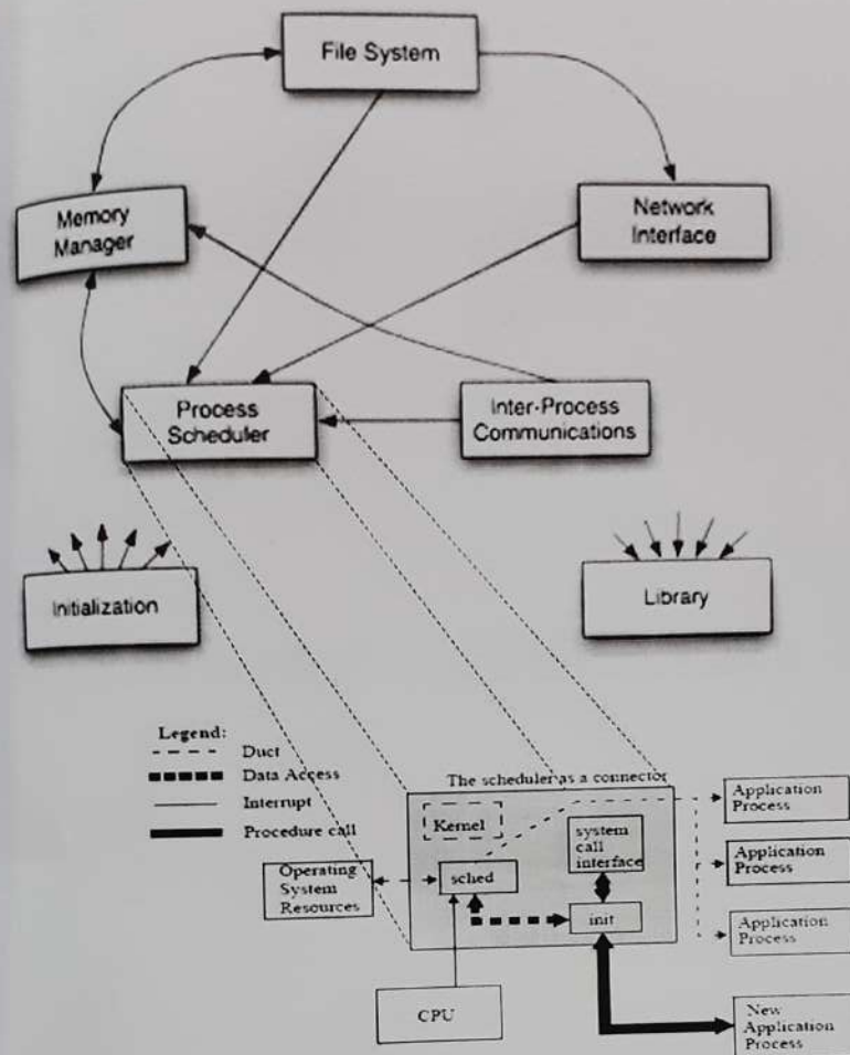
A high level model of the Linux operating system
